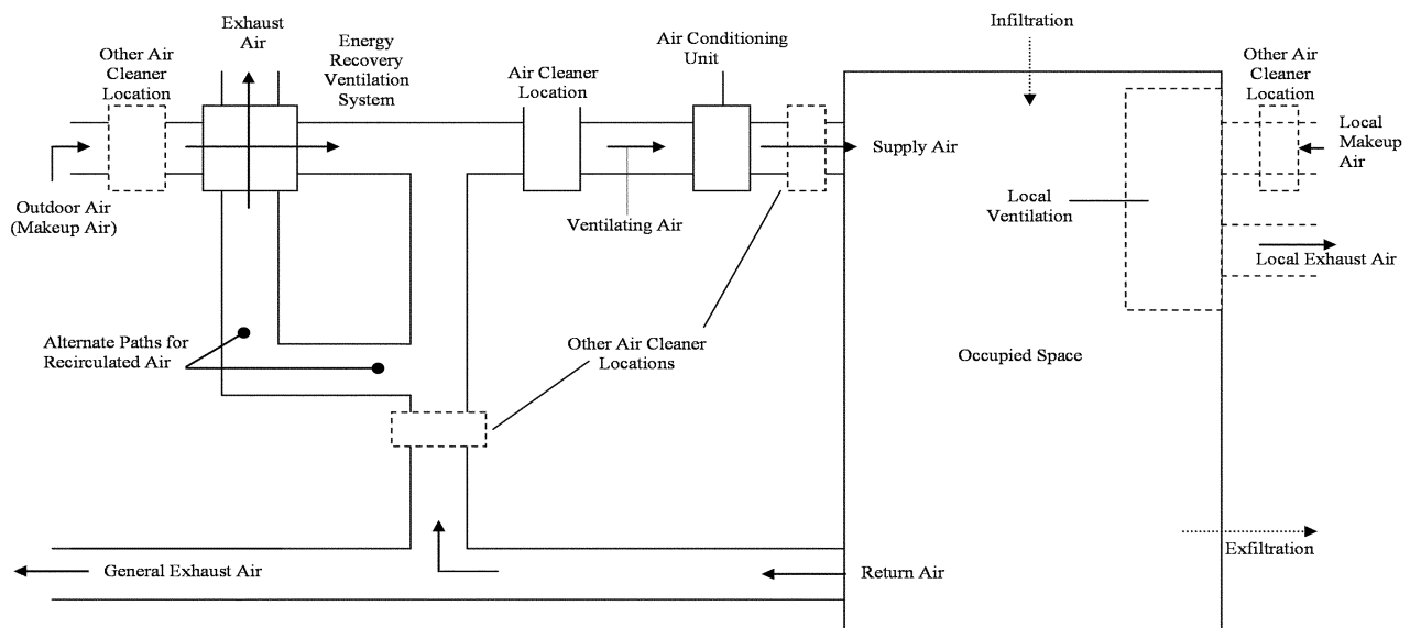
Figure 3.1 Ventilation system.
