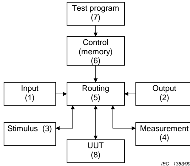
Figure 1 – General configuration of an ATE system
